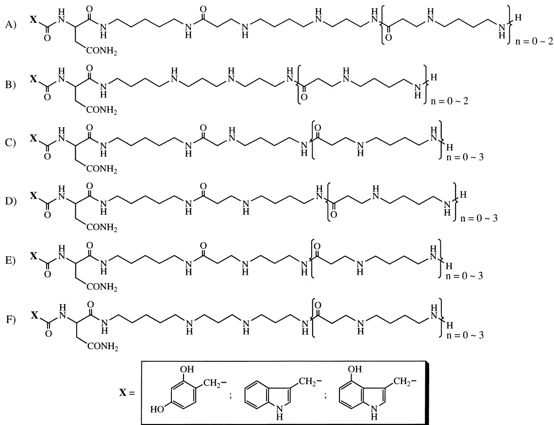
Fig. 2. Classification of acylpolyamine-type spider toxins. In some cases, putreanine unit, -\{\text{COCH}_2\text{CH}_2\text{NH}(\text{CH}_2)_4\text{NH}\}_n\text{H} , is replaced by the arginine residue.
